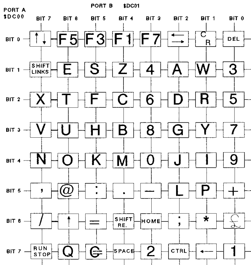
Abb. 3.6: Tastatur-Matrix
